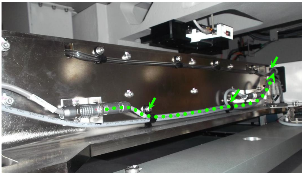
Figure 31 Stepper Motor Cable Routing
