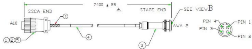
Figure 28 Cable Drawing
