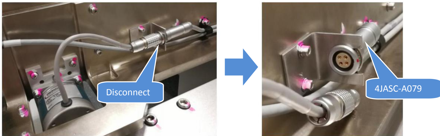
Figure 2 Right Stepper Motor Connector Removal
